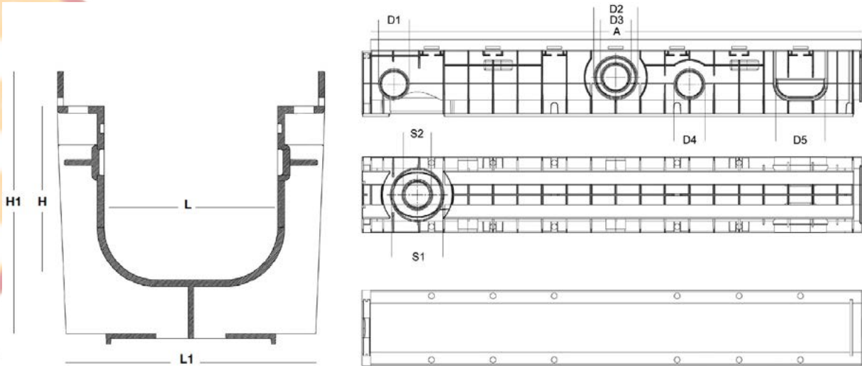
SABDRAIN 370
