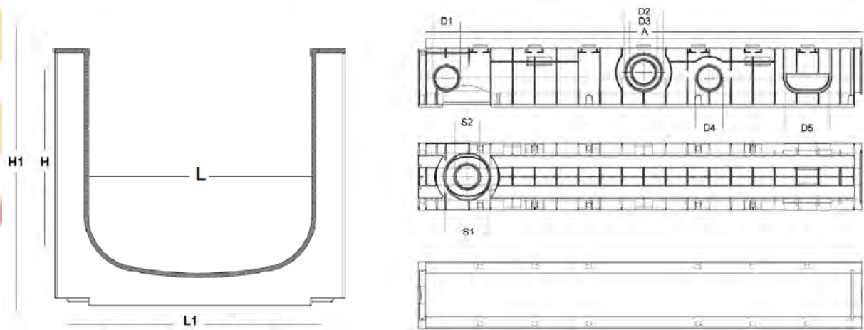
SABDRAIN 952
