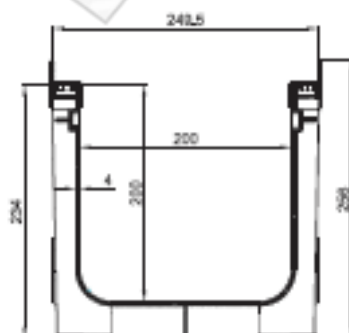
SECTION A-A WITH STEEL EDGE
