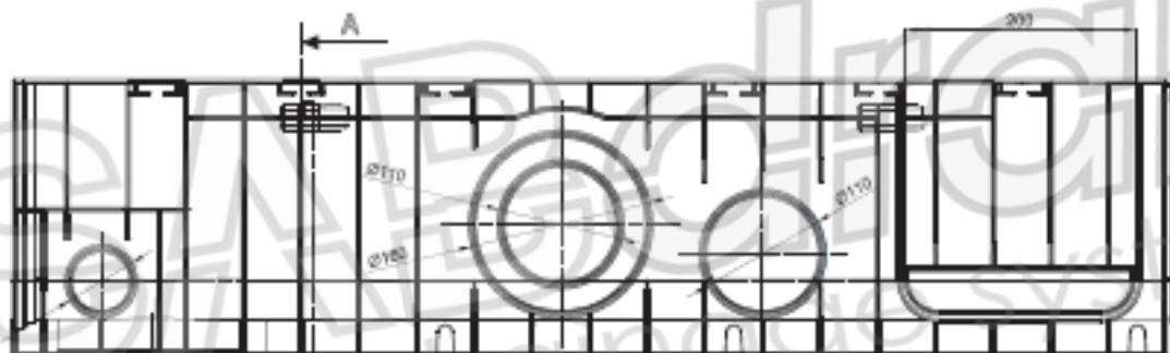
LATERAL VIEW
