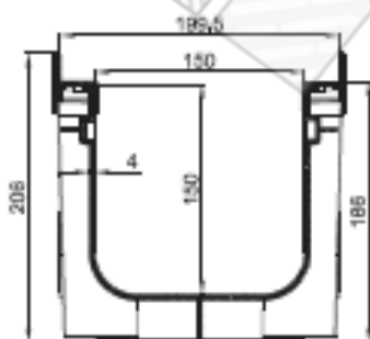
SECTION A-A WITH STEEL EDGE
