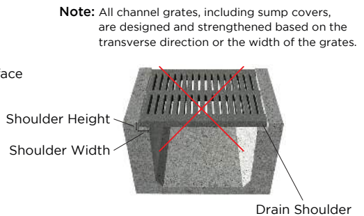
Wrong Orientation for gratings installation.
